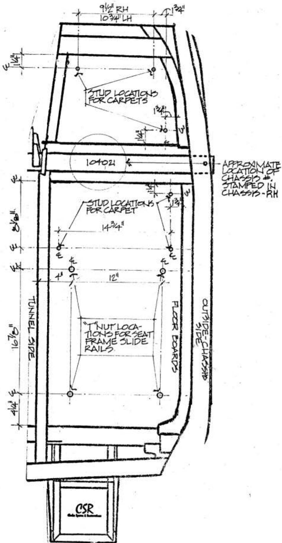
LOCATION DIAGRAM A. 1" NUTS - SEAT FRAME SLIDE RAILS B. SCREW STUDS - CARPET "LIFT-THE-DOT" C. CHASSIS I.D. NUMBER FLOORBOARD SUNDRIES
