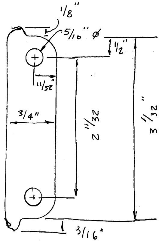
MGA TUNNEL REINFORCEMENT BRACKET (2) Required - - Fits inside tunnel below propshaft at hand brake attachment point
