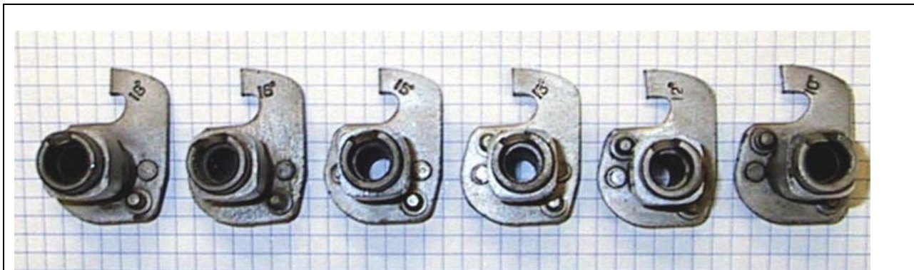
A group of 23D/25D cams ranging from 18° to 10°
